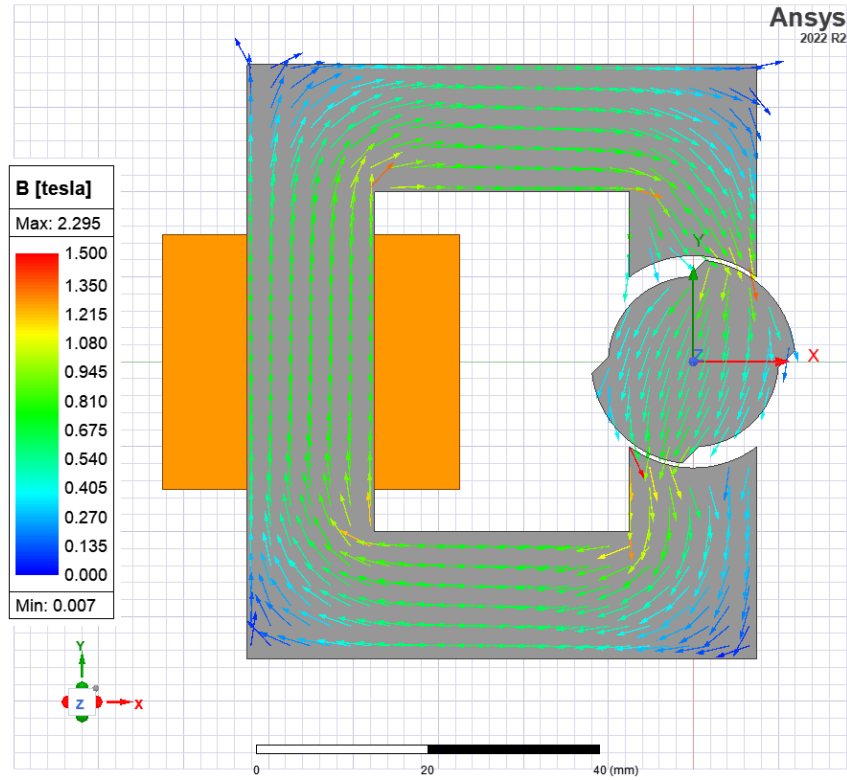
Figure 9: Flux density at 45° for non-linear material
