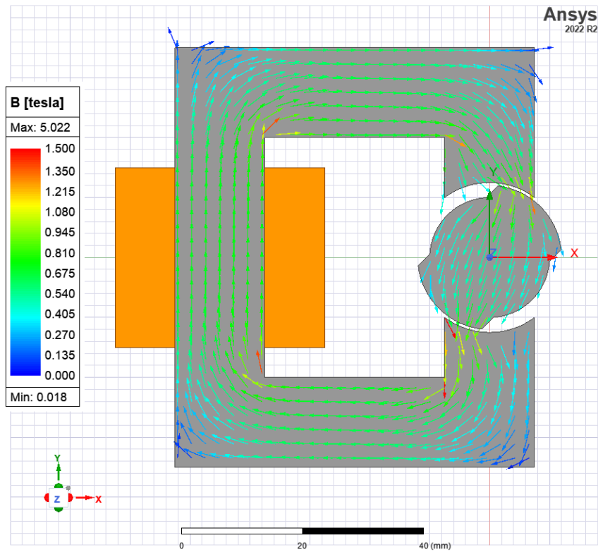
Figure 5: Flux density at 45^\circ for linear material
