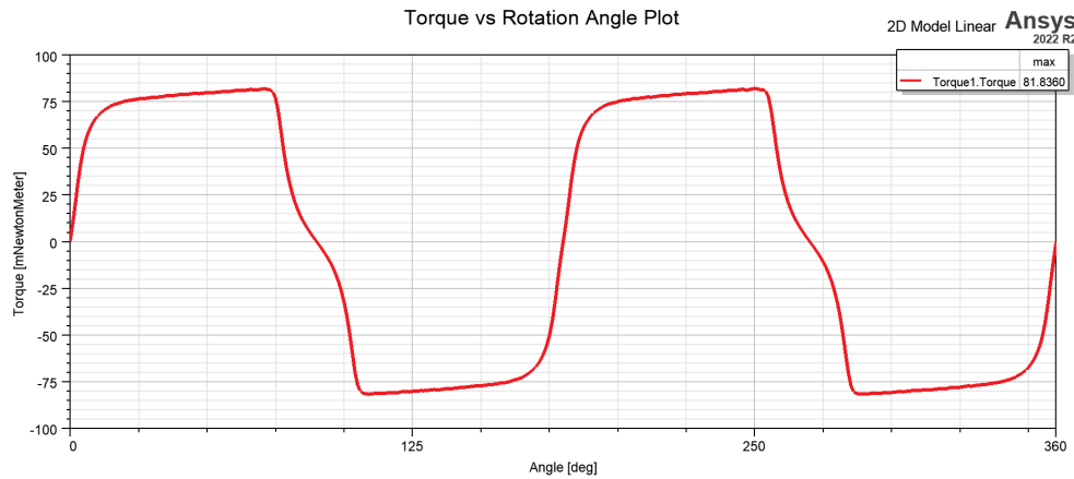
Figure 7: Torque variation with respect to rotor angle from FEA simulations for linear material.
