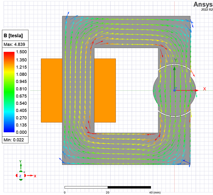
Figure 4: Flux density at 0^\circ for linear material
