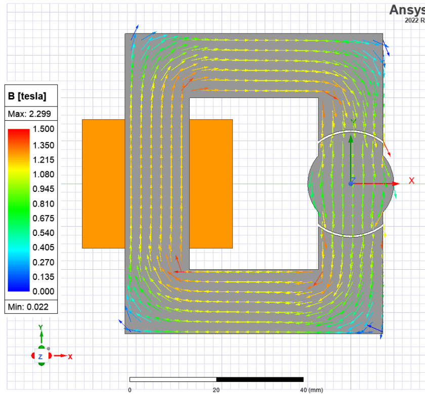
Figure 8: Flux density at 0^\circ for non-linear material
