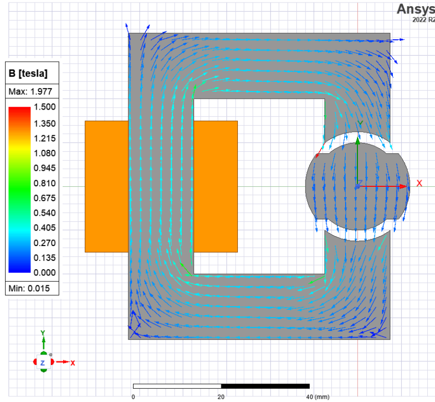
Figure 6: Flux density at 90^\circ for linear material
