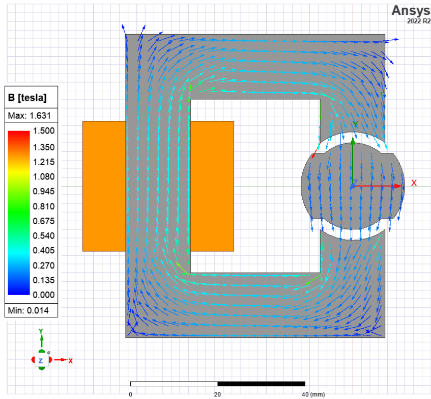
Figure 10: Flux density at 90° for non-linear material
